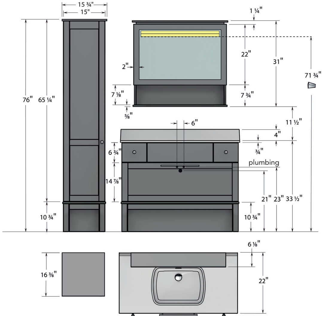
DIMENSIONS OF THE EVOLO SINK
