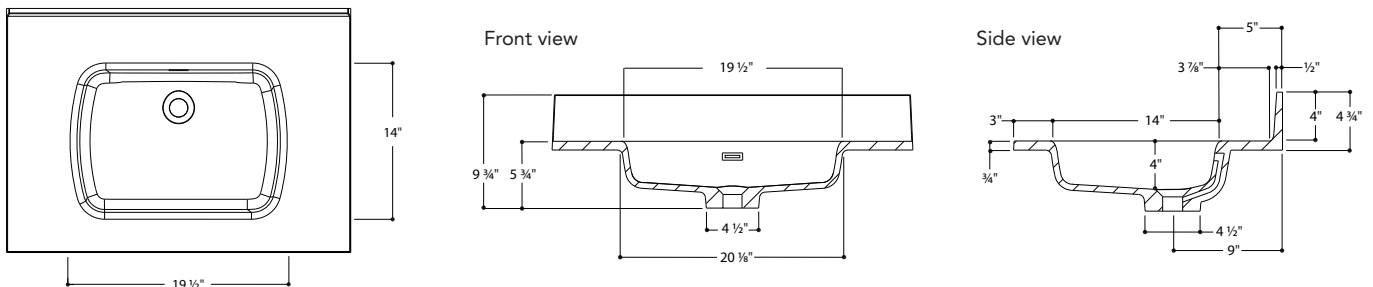
DIMENSIONS OF THE EVOLO SINK
