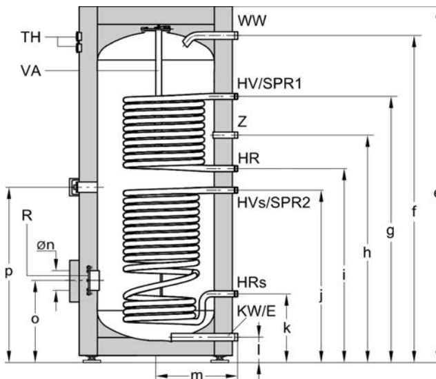
Tank 119 USG (450 L) Dimensions
