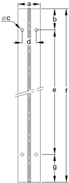
Base rail hole dimensions
