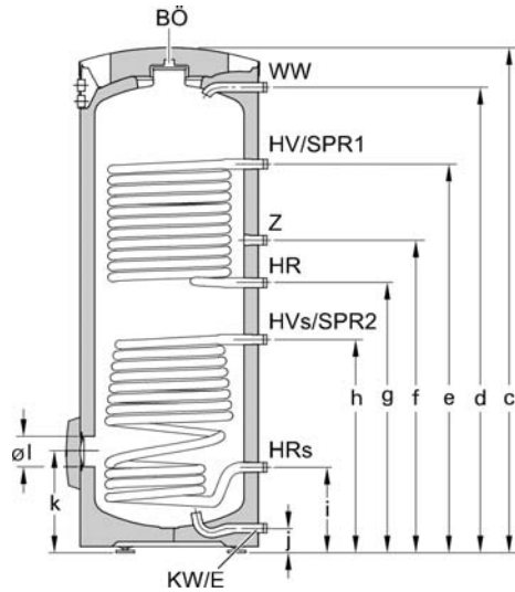
Tank 79 USG (300 L) Dimensions
