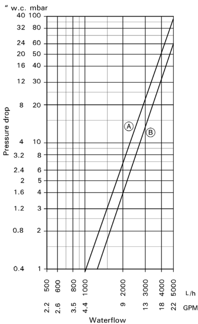
Domestic hot water pressure drop
