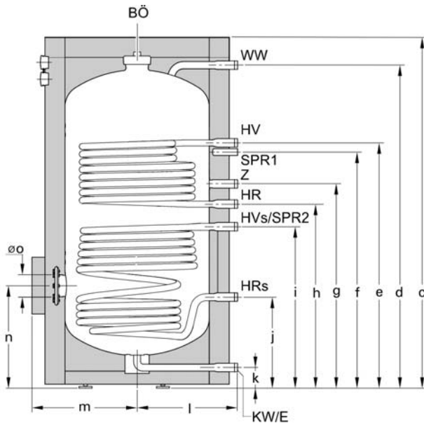
Tank 119 USG (450 L) Dimensions
