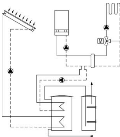
System with dual coil heating buffer tank and a direct fire DHW tank
