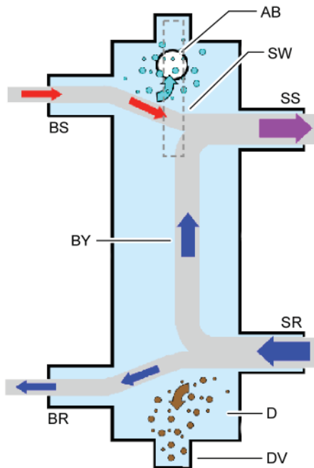
Low-loss header design (Typical)
