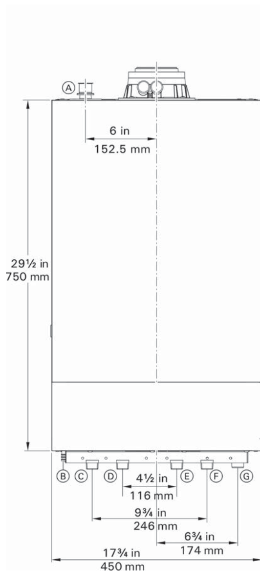
Front view
