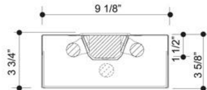
248 - 2 or 3 LAMP
