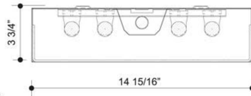
248 - 2 or 3 LAMP
