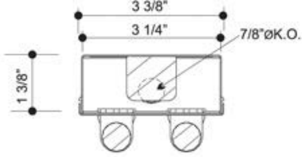
Standard Two Lamp T5
