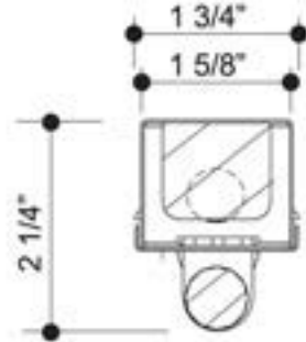
Standard One Lamp T5
