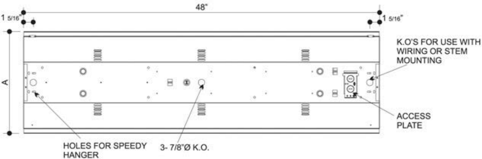
Back View
