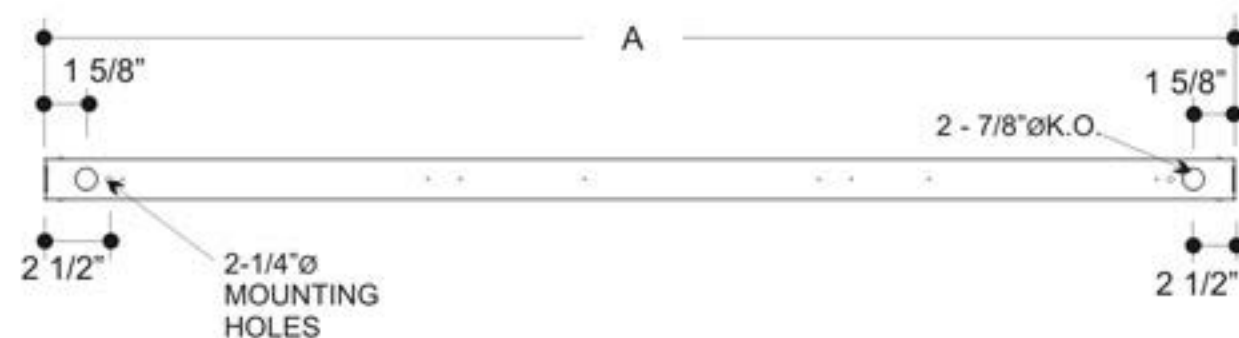
Back View 1 Lamp
