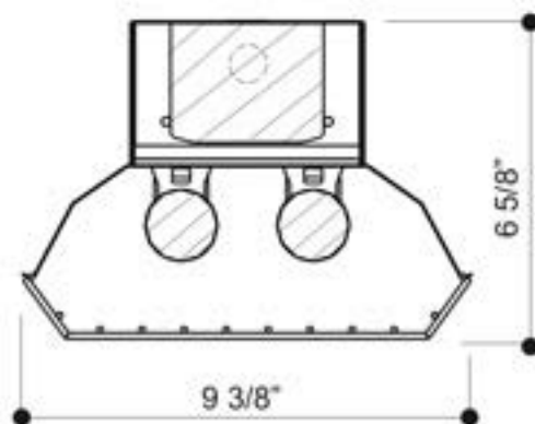
Cross Sections
