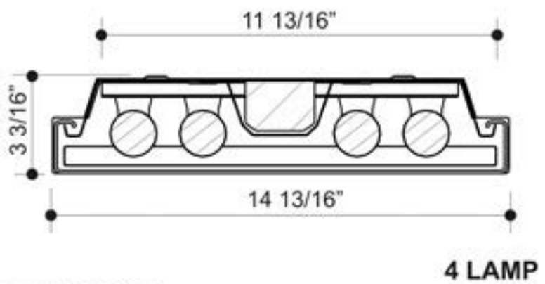
Cross Sections
