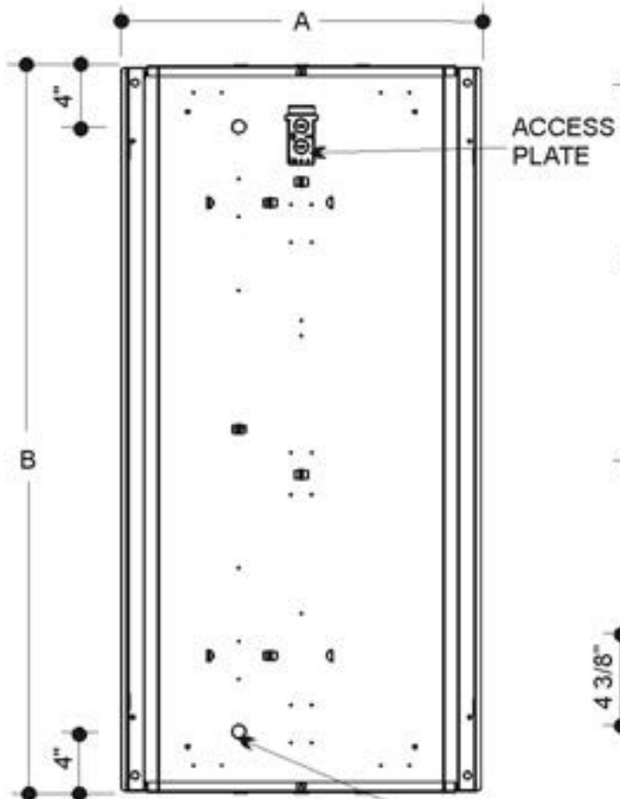
Back View
