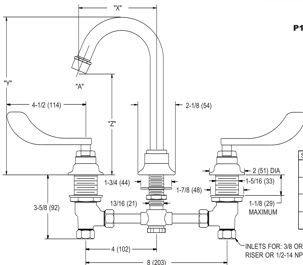
Gooseneck Spout Dimensions
