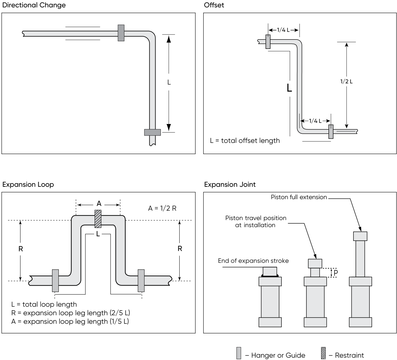
Figure 3 - Pipe Configurations for Expansion/Contraction
