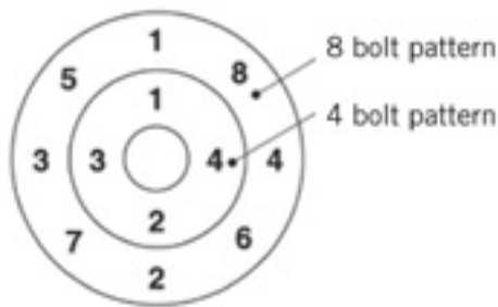
Figure 1: Tightening Sequence
