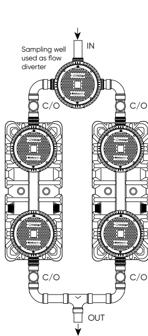
2 XL 100 – PARALLEL Up to 200 GPM, 2116 lbs Grease Capacity. 2 XL 150 – PARALLEL Up to 300 GPM, 2194 lbs Grease Capacity.
