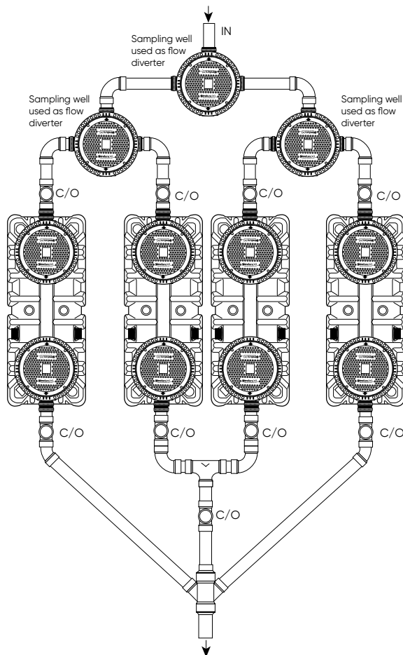
4 XL 100 – PARALLEL Up to 400 GPM, 4232 lbs Grease Capacity. 4 XL 150 – PARALLEL Up to 600 GPM, 4388 lbs Grease Capacity.
