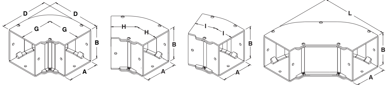
ELBOW 90°
