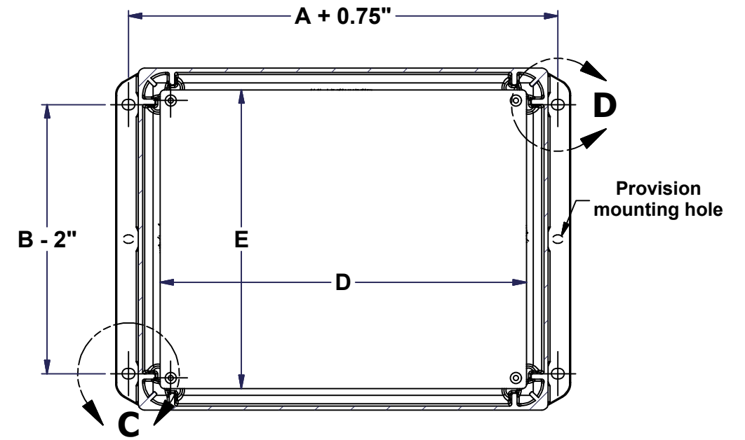
SECTION B-B Mounting feet type 1 (060404 to 141208)
