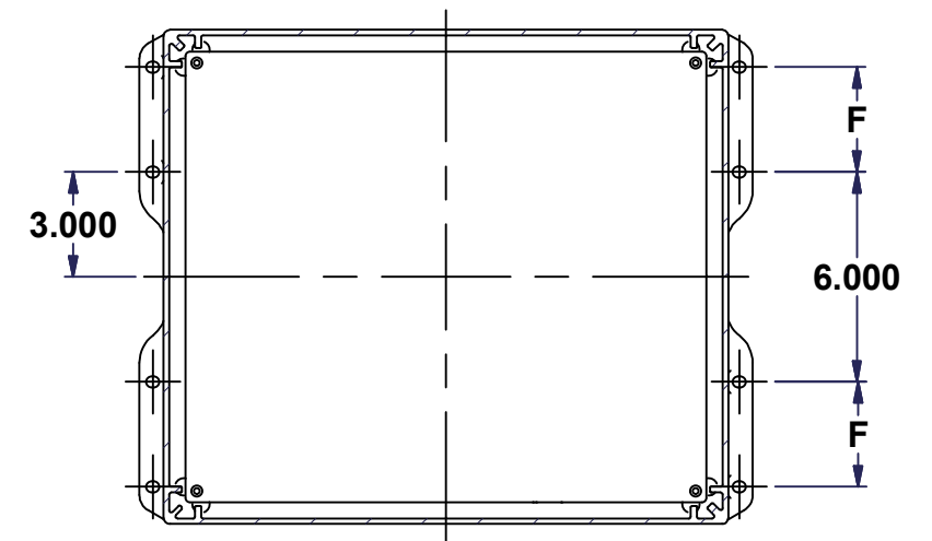
Mounting feet type 2 (161406 to 201606)
