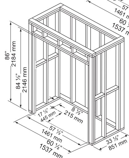
FIGURE 1 - LAYOUT DIMENSIONS
