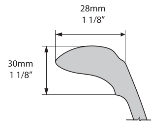
Rim detail
