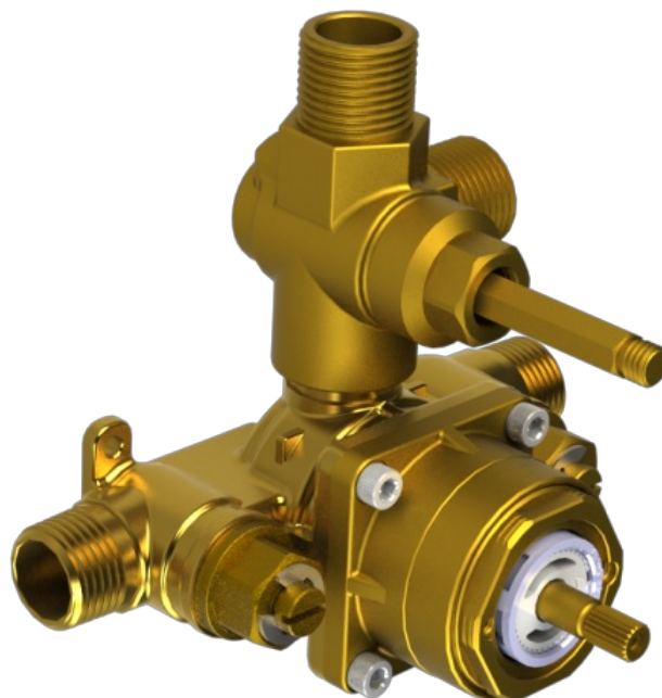
VALVE ONLY PRESSURE BALANCE WITH DIVERTER AND STOPS ROUGH-IN
