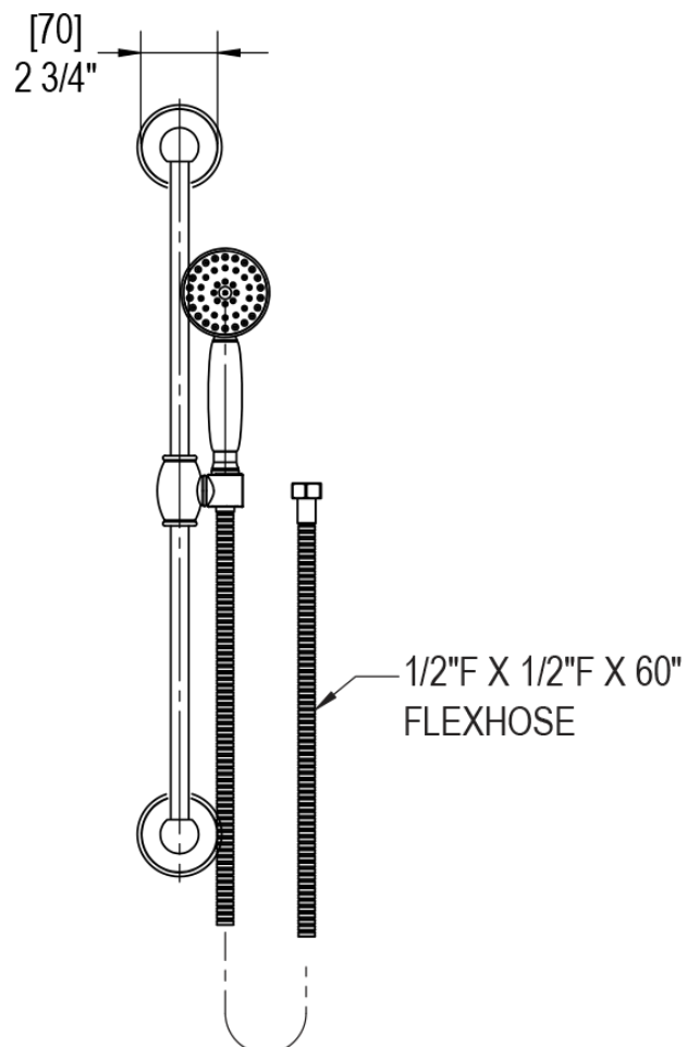
Adjustable Slide Bar with Hand Held Shower Assembly (Single Function)
