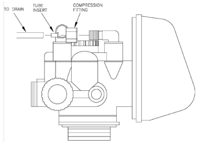
Figure 12: Drain Line Connection
