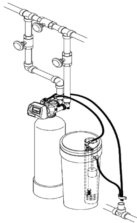
Figure 2: Plumbing with 3 valve bypass.
