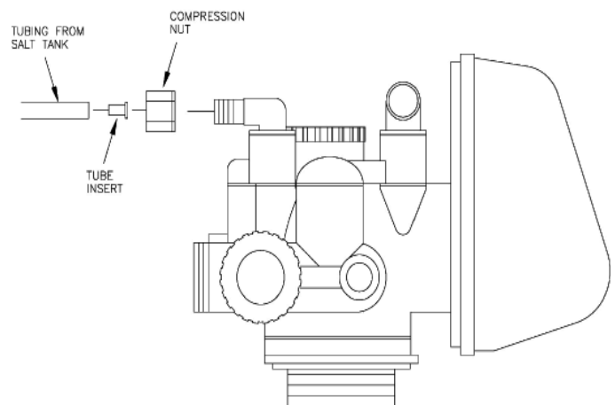
Figure 9: Brine Draw Connection
