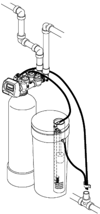
Figure 1: Plumbing with by pass (STANDARD).
