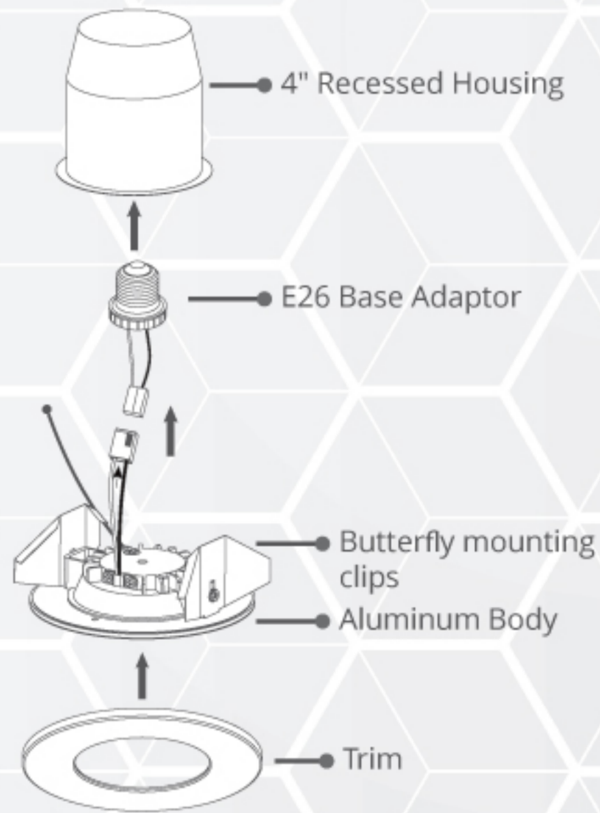
4" Recessed Housing
