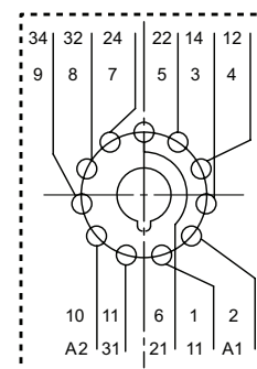
Wiring Diagram
