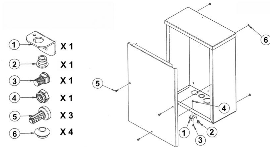
Enclosure Assembly Illustrative Diagram
