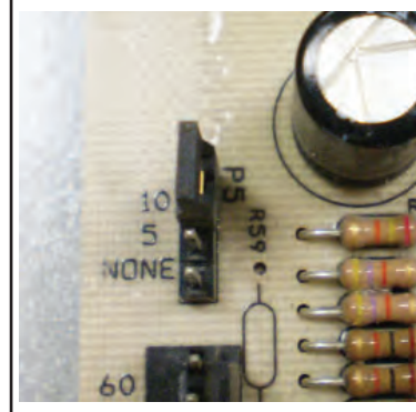
FIGURE 32 - JUMPER P5
