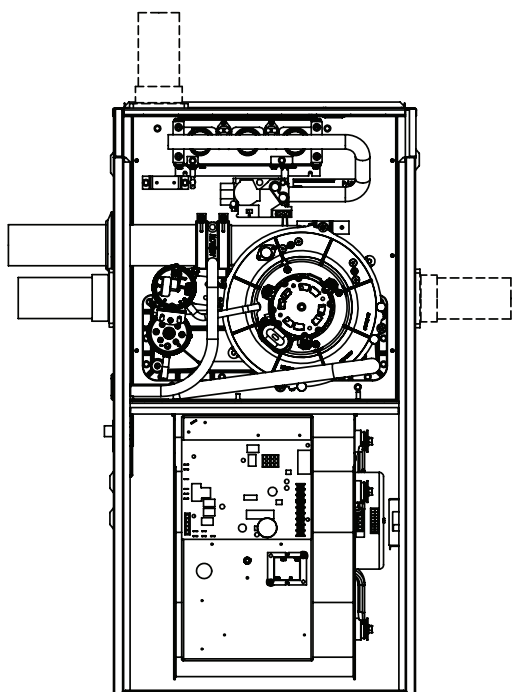
FIGURE 16 - UPFLOW VENT AND DRAINING OPTION
