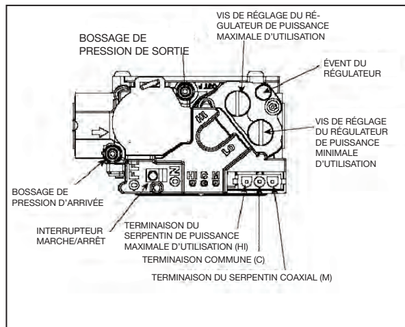
FIGURE 31 - SOUPAPE DE GAZ WHITE RODGERS 36G54
