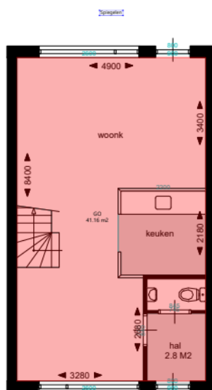
Begane_grond
