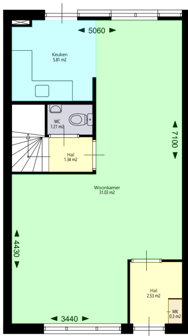
Begane_grond
