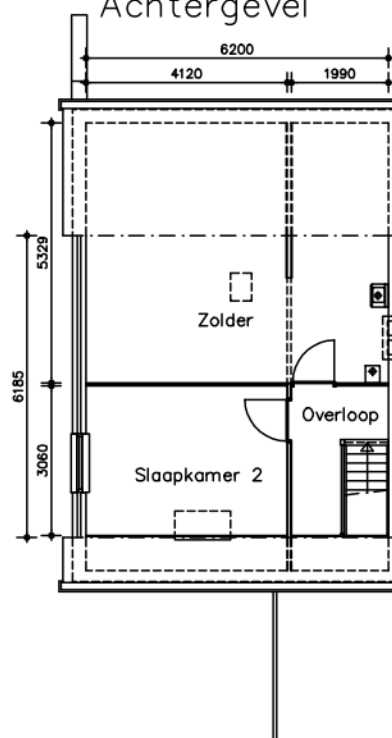
Zolder
