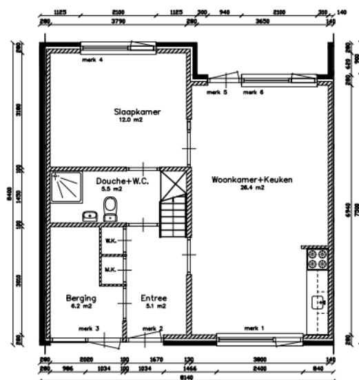
Begane-grond
