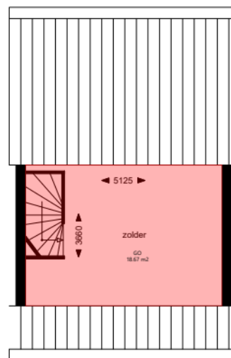
Zolder
