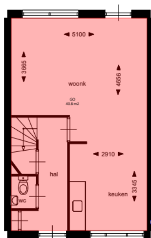
Begane_grond
