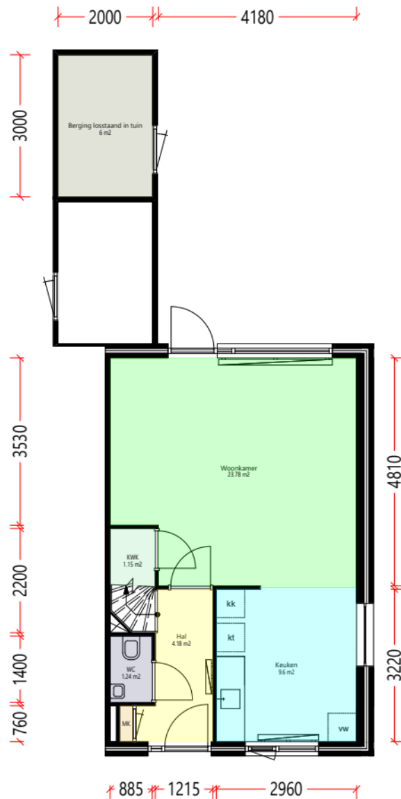
Begane_grond
