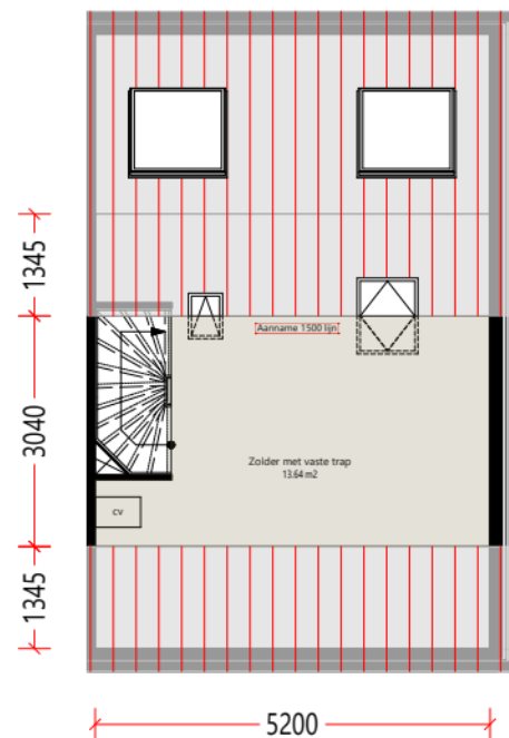
Zolder
