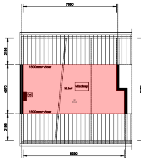
Zolder
