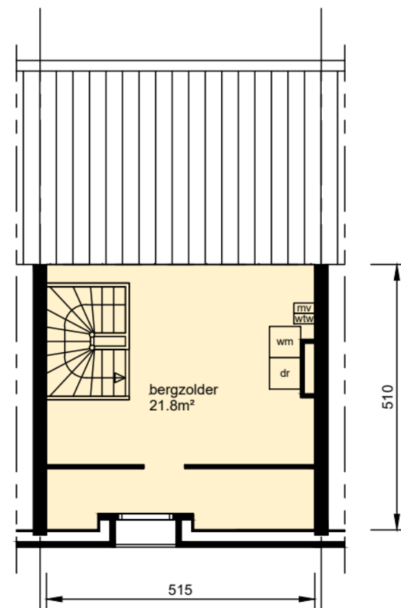
zolder
