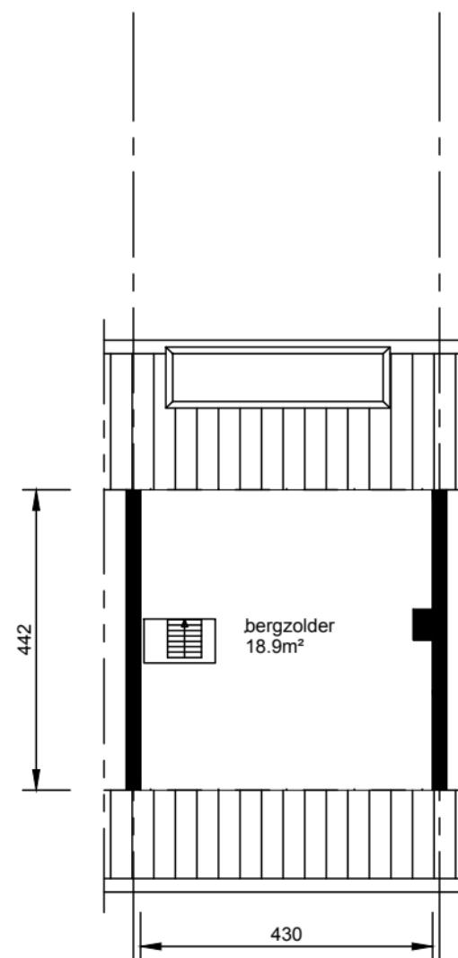
zolder
