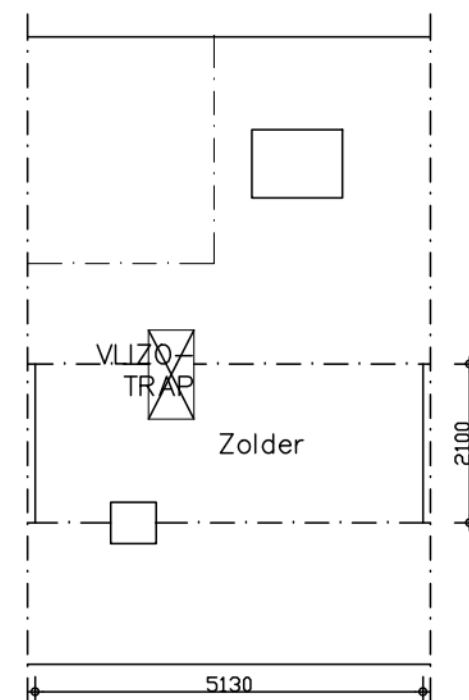
Zolder
