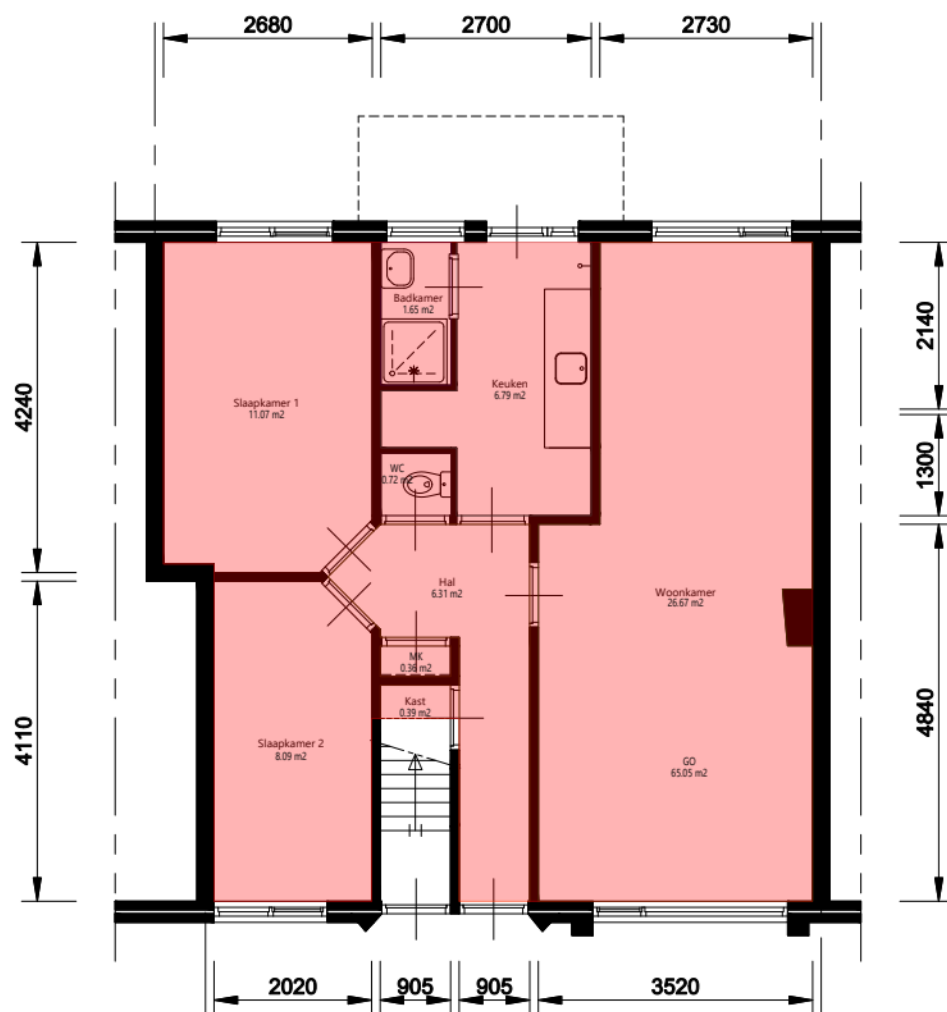
Begane_grond
