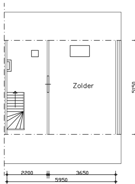
Zolder
