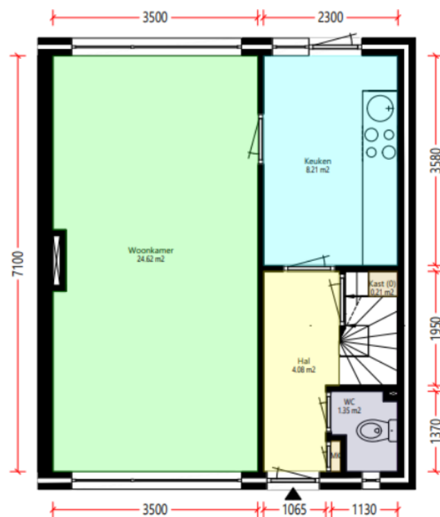
Begane_grond
