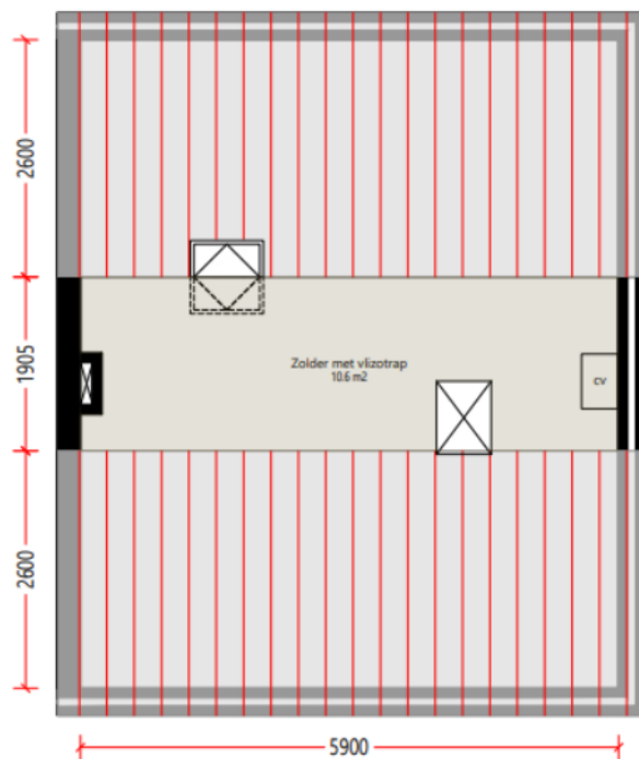
Zolder
