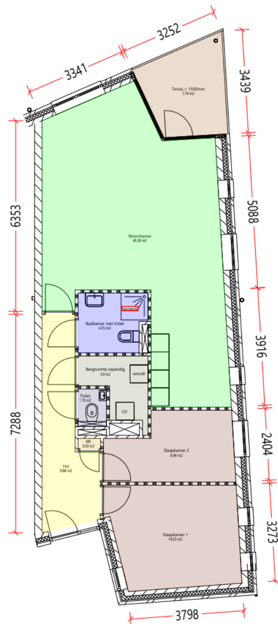
Begane_grond
