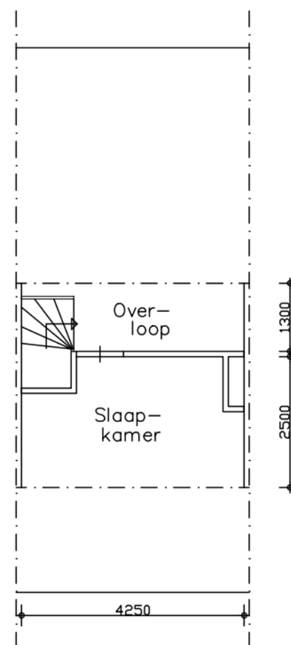
Zolder
