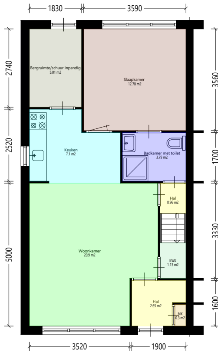
Begane_grond
