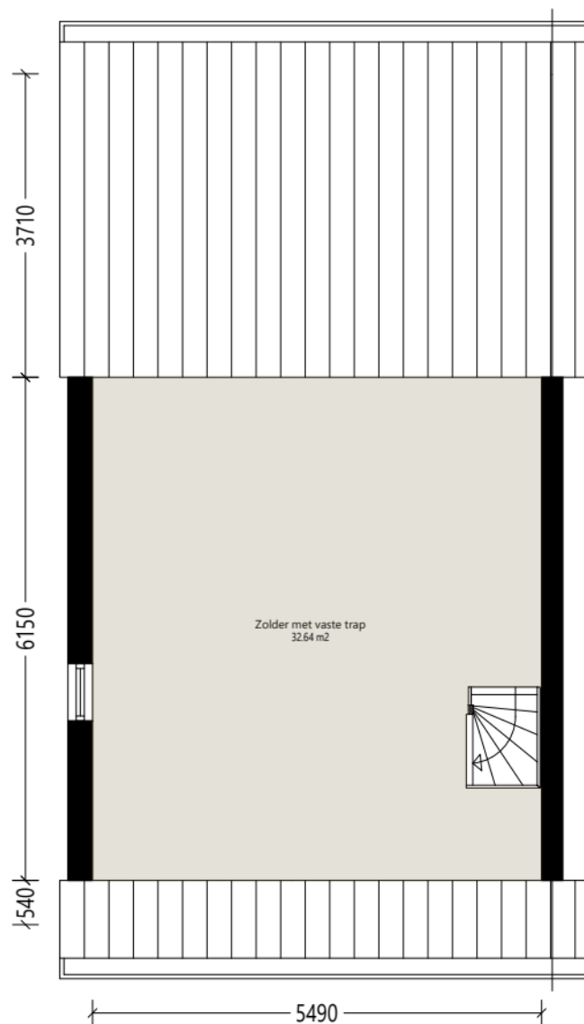
Zolder
