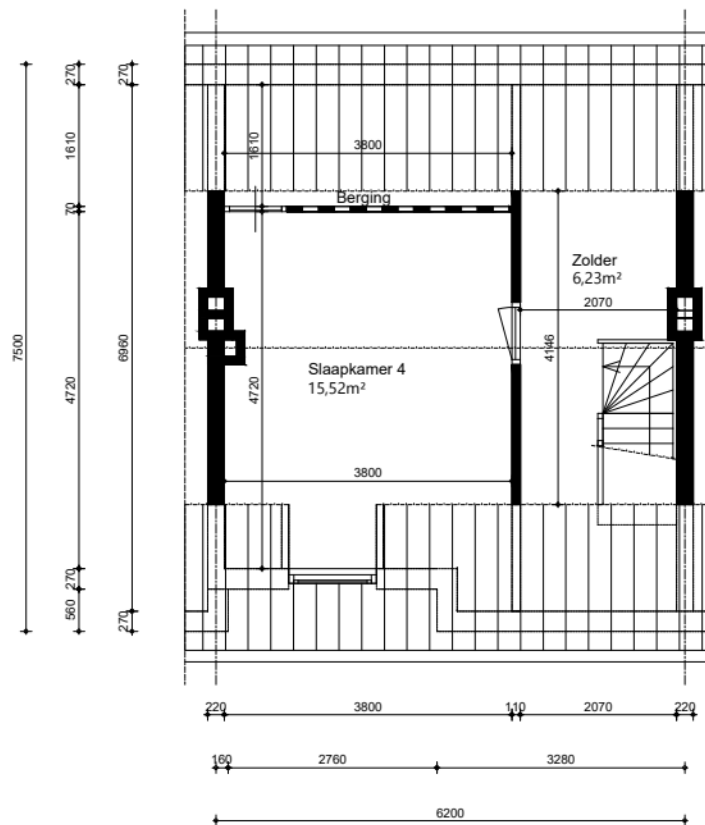
Zolder
