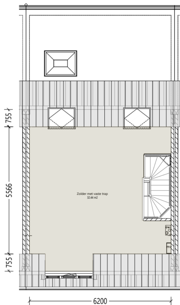
Zolder
