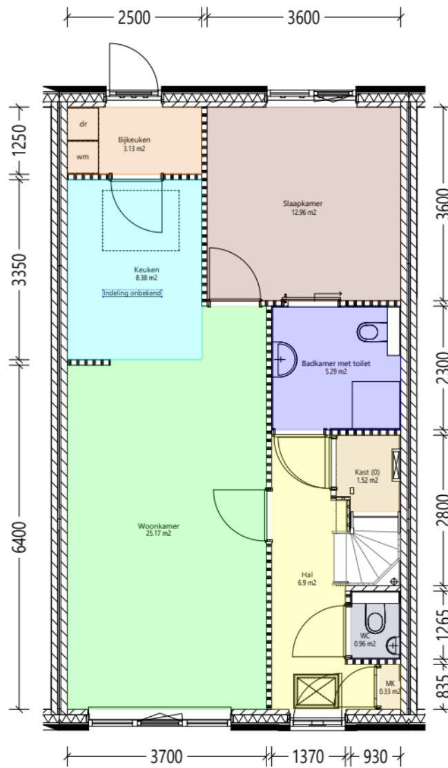
Begane_grond
