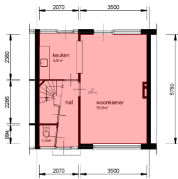
Begane_grond
