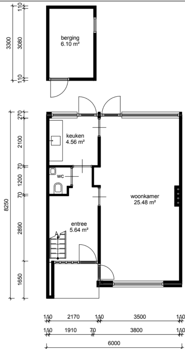
Begane Grond GBO: 47.74 m²
