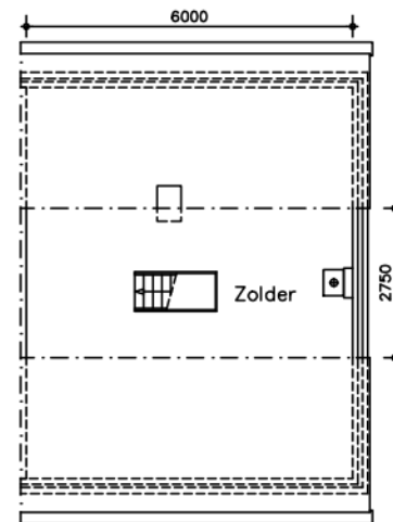
Zolder
