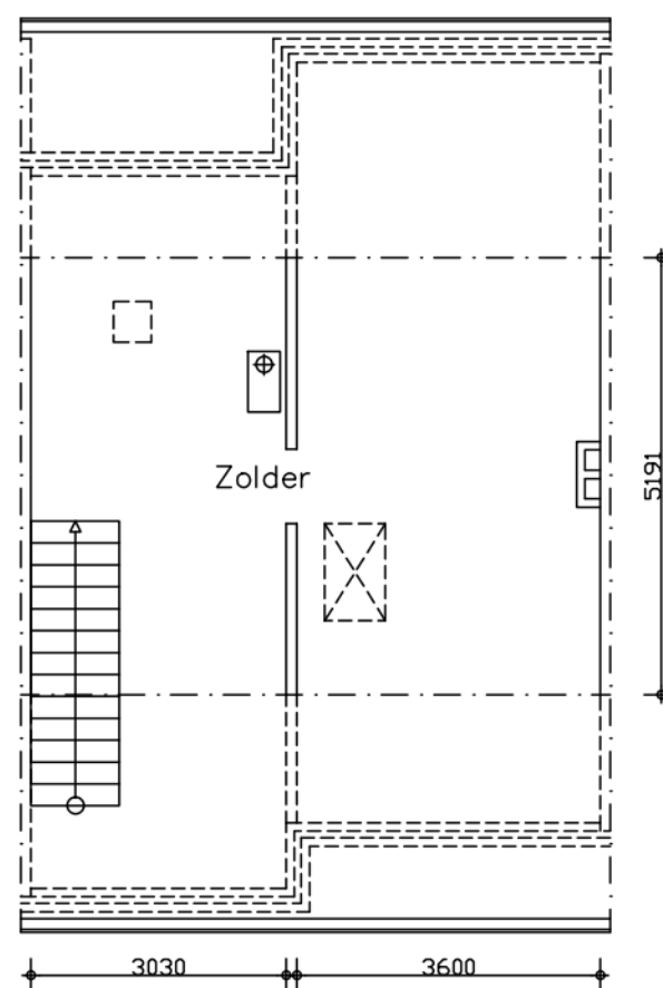
Zolder
