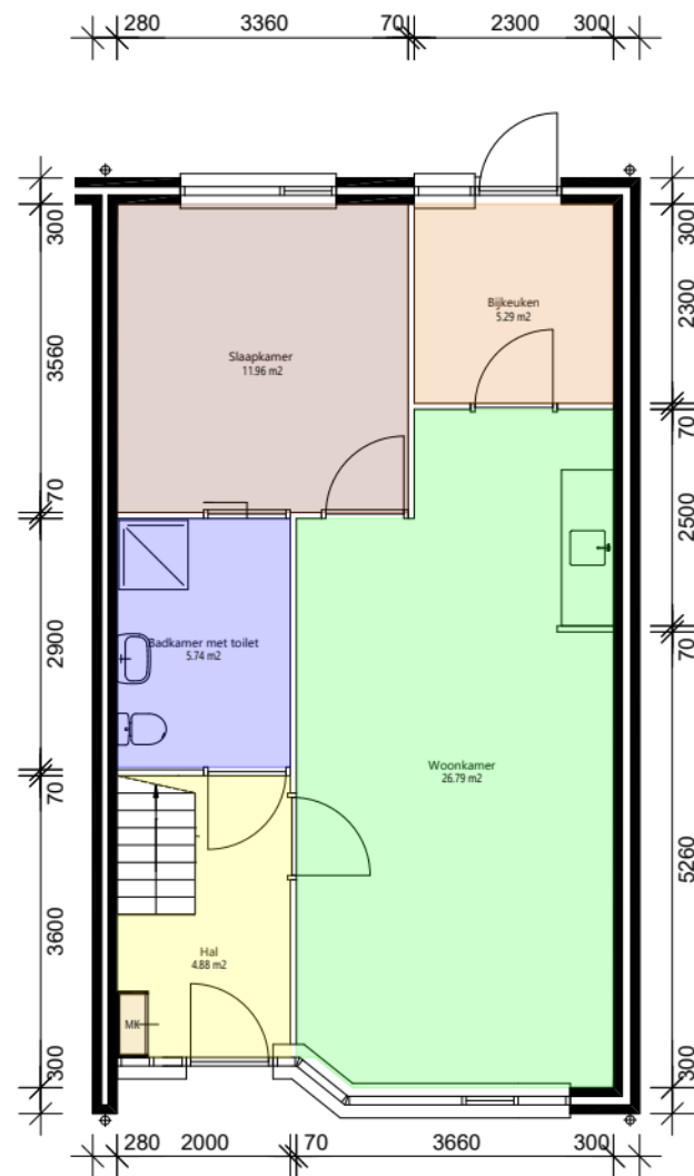
Begane_grond
