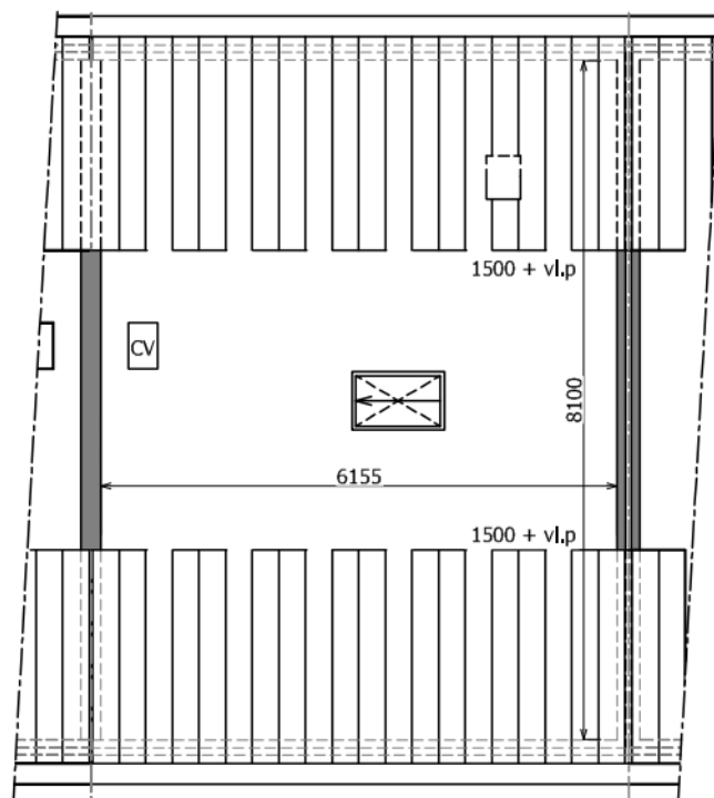
Zolder
