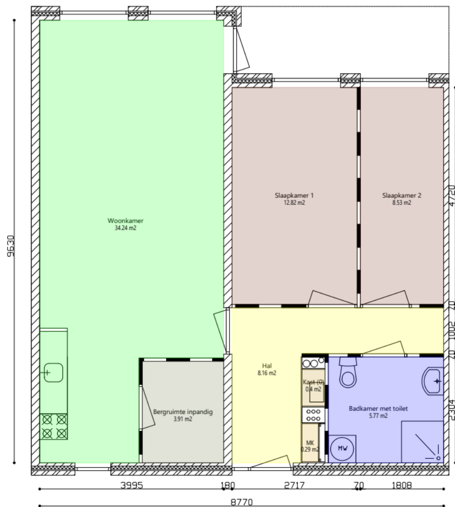
Begane_grond
