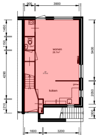
Begane_grond
